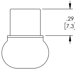
"P1" USB TYPE C MALE CONNECTOR
