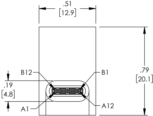
"P1" USB TYPE C MALE CONNECTOR
