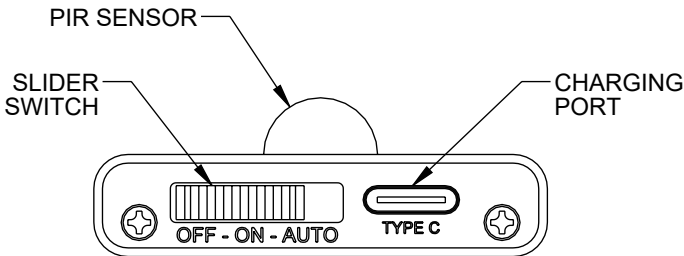
DETAIL A ROTATED 90° CW
