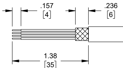
RECOMMENDED STRIPPING DIMENSIONS
