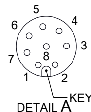
M12 MALE 8 PIN A-CODED CONNECTOR OUTSIDE VIEW
