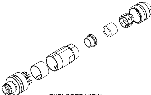
EXPLODED VIEW
