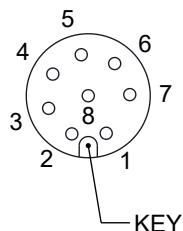
DETAIL A OUTSIDE VIEW
