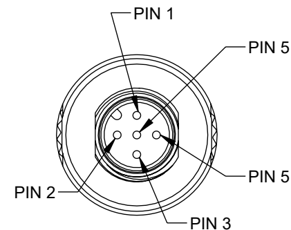
M12 MALE 5 PIN A-CODED CONNECTOR
