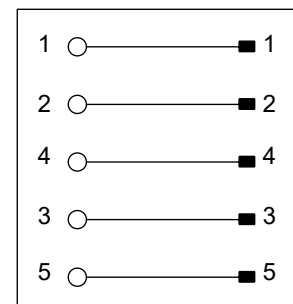
SPlicing RING M12 MALE
