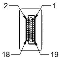
P1 HDMI 19P MALE CONNECTOR INSULATION: BLACK PINS & SHELL: GOLD PLATED
