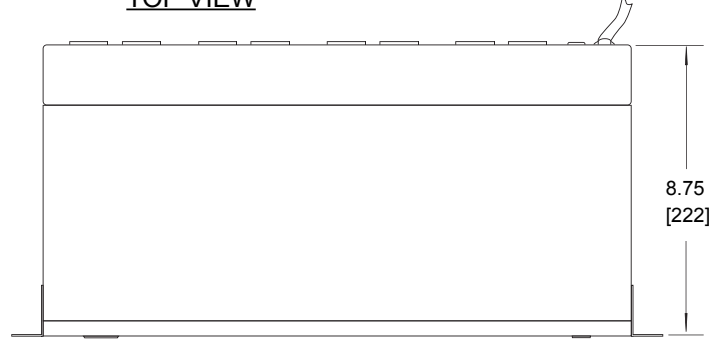
REAR VIEW
