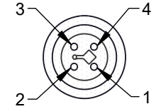
P2 M12 FEMALE T-CODED 4PIN CONNECTOR
