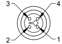
P2 M12 FEMALE T-CODED 4PIN CONNECTOR
