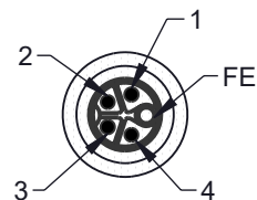
P1 M12 MALE K-CODED 5PIN CONNECTOR
