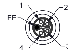
P2 M12 FEMALE K-CODED 5PIN CONNECTOR
