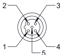
P1 M12 FEMALE B-CODING 5 POSITION
