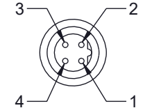
P2 M12 MALE B-CODING 4 POSITION
