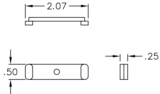
MOUNTING CLIP
