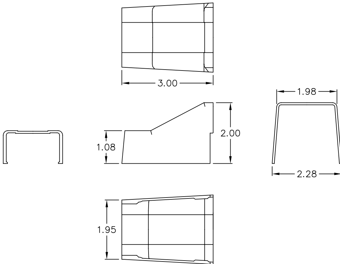
3/4" CEILING ENTRY
