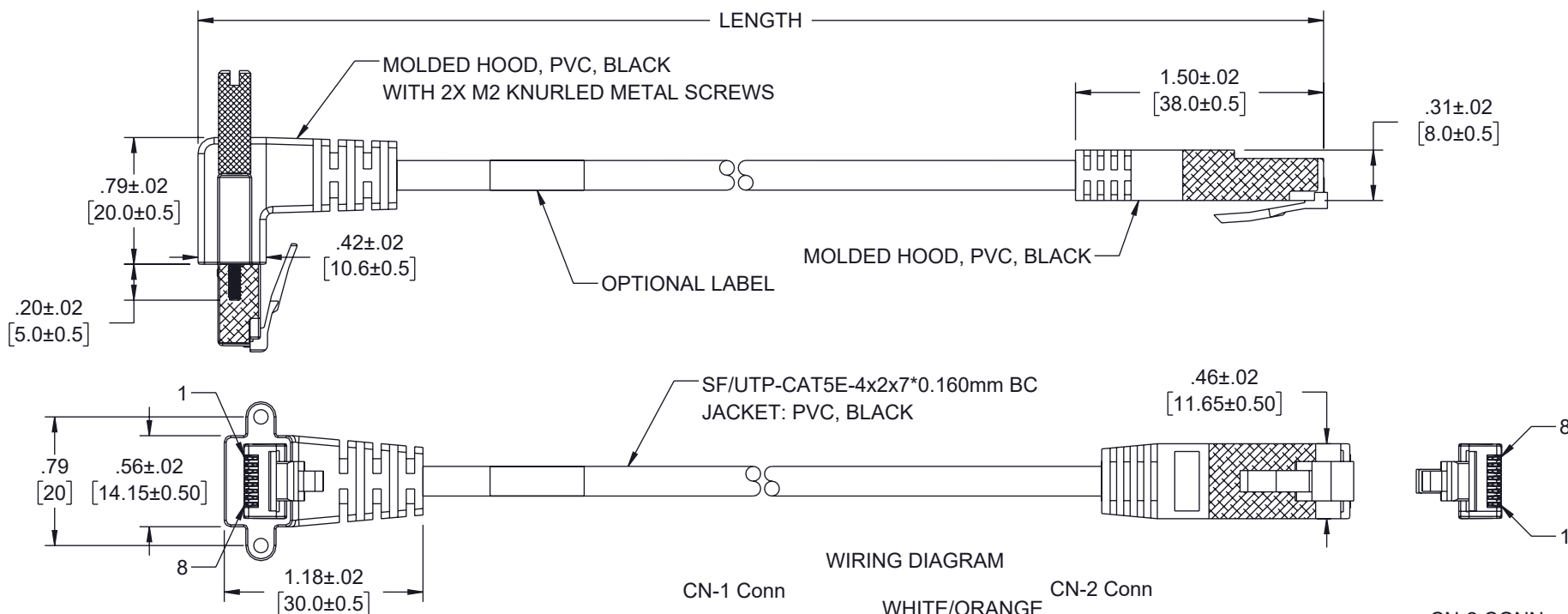
CN-1 CONN SHIELDED RJ45 PLUG GOLD-PLATED CONTACTS (8P8C)
