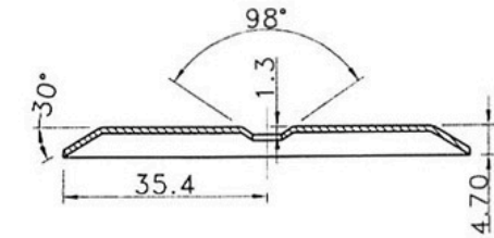
D-SUB 15 SINGLE HOLE STAINLESS WALL PLATE
