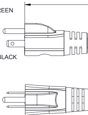
N5-15 MALE PLUG NICKEL PLATED TERMINALS
