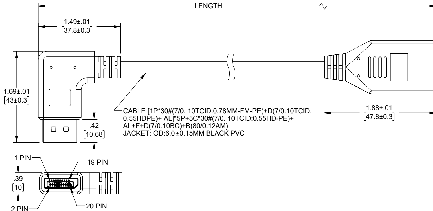
P1 DP20P M PLUG LEFT ANGLE GOLD PLATED
