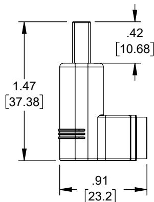
P1 DP20P M PLUG DOWN ANGLE GOLD PLATED
