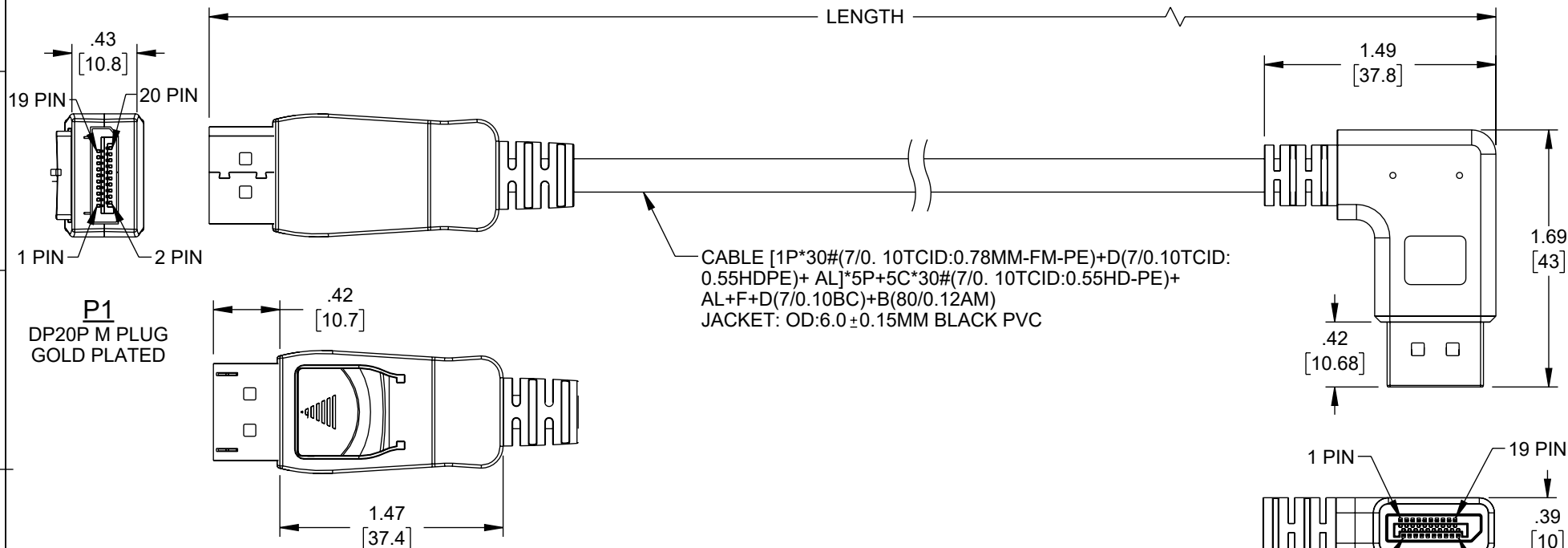
P2 DP20P M PLUG RIGHT ANGLE GOLD PLATED
