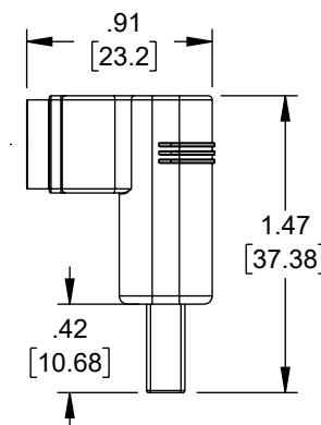
P2 DP20P M PLUG DOWN ANGLE GOLD PLATED
