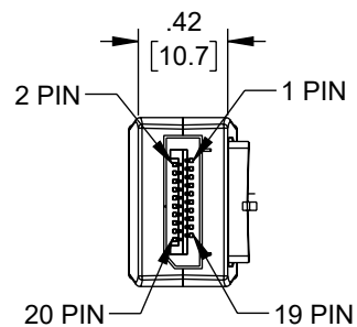
P1 DP20P M PLUG GOLD PLATED
