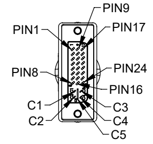
P2 DVI29 MALE, GOLD PLATING CONTACTS CONNECTOR
