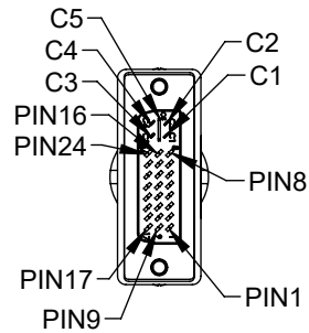
P1 DVI29 MALE, GOLD PLATING CONTACTS CONNECTOR
