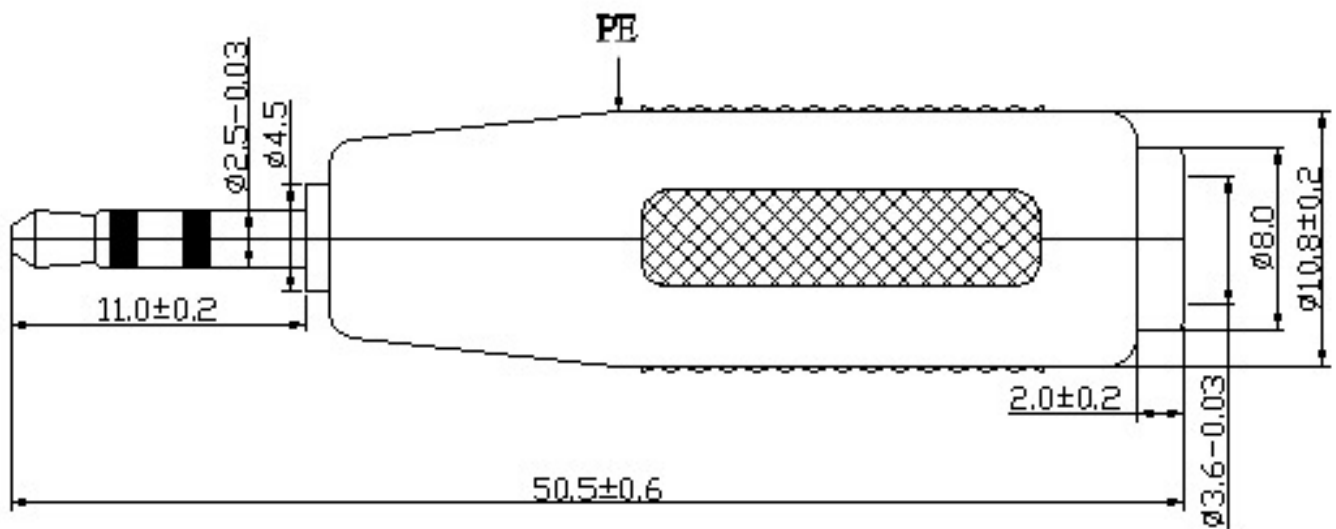
3.5mm stereo jack to 2.5mm stereo plug
