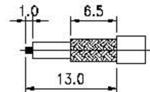
STRIPPING DIMENSION
