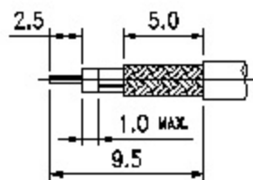
STRIPPING DIMENSION
