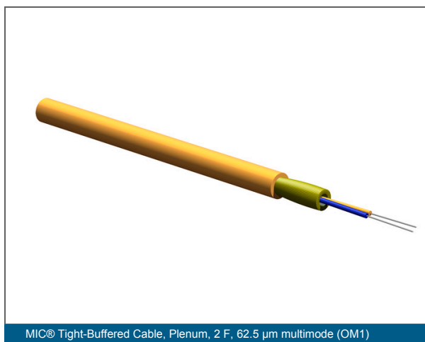
MIC® Tight-Buffered Cable, Plenum, 2 F, 62.5 µm multimode (OM1)
