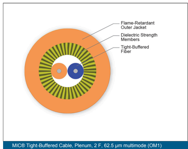
MIC® Tight-Buffered Cable, Plenum, 2 F, 62.5 µm multimode (OM1)
